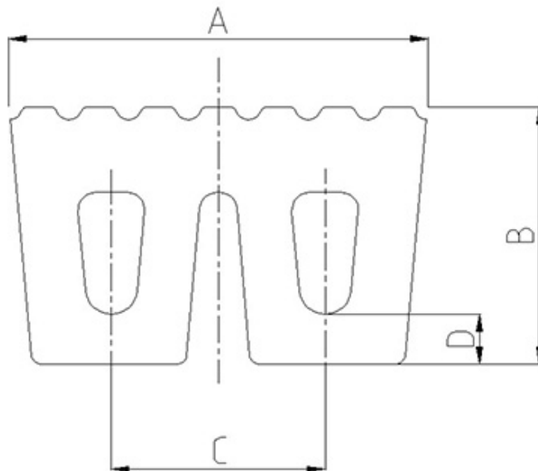
Figure 1 The structure of W-type fender
